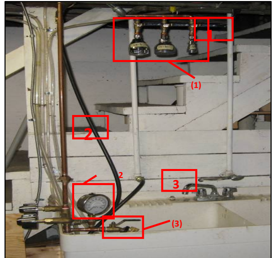
Figure 4: Test rig with (1) multiple showerheads, each with their own shutoff valve; (2) a pressure gauge; and (3) a throttling valve to simulate various tub spout leak sizes
